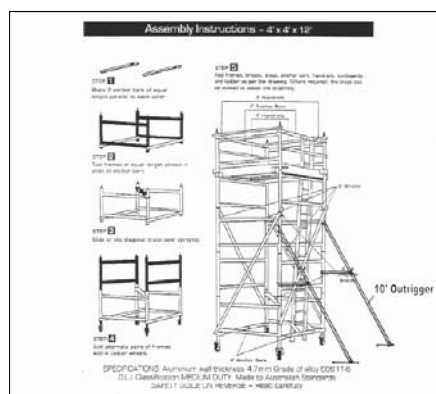
Examples of suppliers' erection instructions
